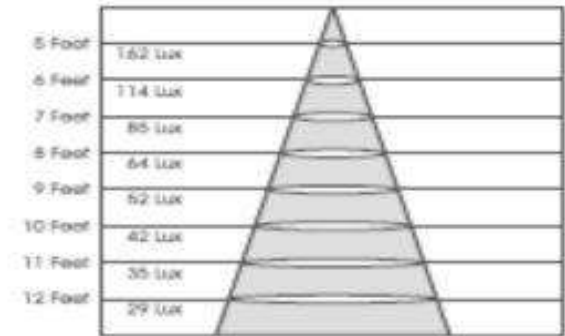
Lux-Distance Curve
